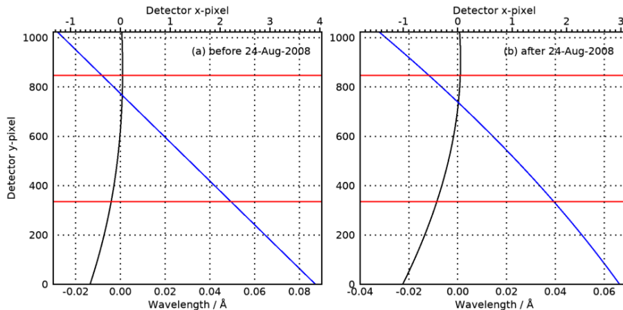
Figure 5. Comparisons of the 1'' slit ( black ) and the centroid of the 40'' slit ( blue ) as they appear on the EIS detectors. Panels (a) and (b) show the positions prior to and after the grating movement on 24 August 2008, respectively. The red horizontal lines indicate the portion of detector that is most actively used.
