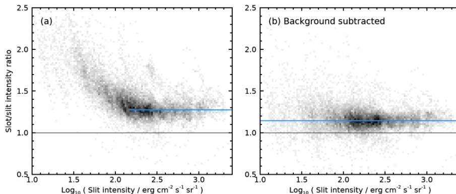
Figure 6. Heatmaps showing ratios of slot to slit intensities for the May 2007 SYNOP001 datasets, plotted as a function of the slit intensity. The bin sizes are 0.02 in both dimensions, and the maximum values are 53 (a) and 56 (b). For display purposes the maps are shown scaled to the power 0.7. Panel (b) shows the effect of background subtraction for the slot intensities. The blue horizontal line on Panel (a) shows the mean ratio value for slit intensities \geq 150 \text{ erg cm}^{-2} \text{ s}^{-1} \text{ sr}^{-1} , and that on Panel (b) shows the mean ratio value for all slit intensities.
