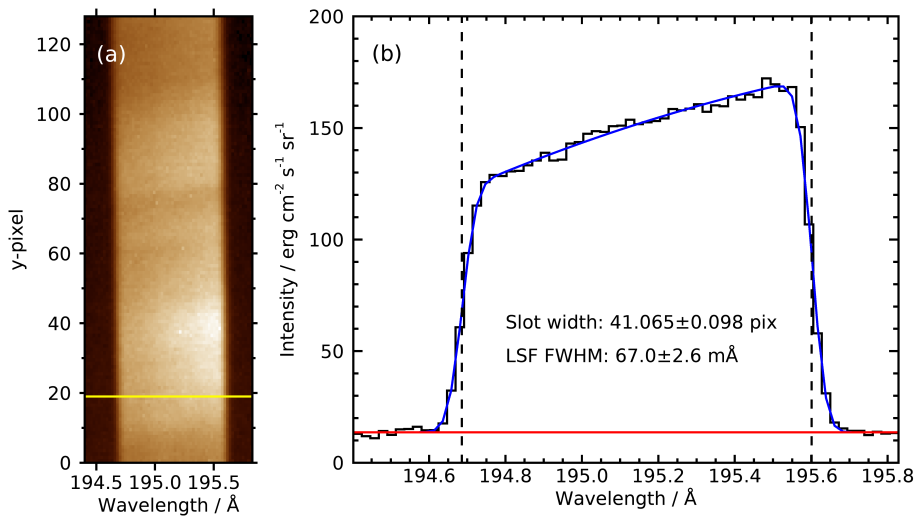
Figure 3. (a) the Fe XII \lambda 195.12 slot image obtained at 13:12 UT on 20 September 2021. (b) the intensity cross-section through the slot image at y-pixel 19 (indicated by the yellow line on Panel a). The blue line shows the seven-parameter fit to the intensity, the horizontal red line shows the fitted background intensity, and the vertical dashed lines show the edges of the slot as derived from the fit.
