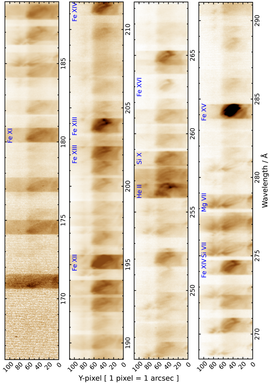
Figure 1. A complete EIS spectrum obtained with the 40'' slot, derived from an observation on 15 May 2007 at 05:41 UT. An inverse, square-root intensity scaling has been applied and an artificial saturation to bring out the weaker features.
